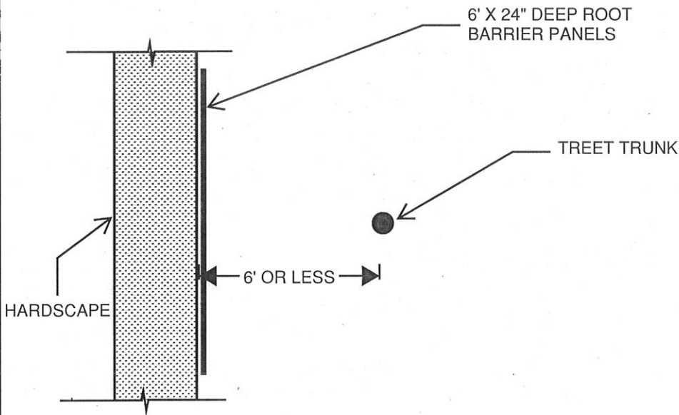
CIRCULAR ROOT BARRIER - PLAN VIEW
