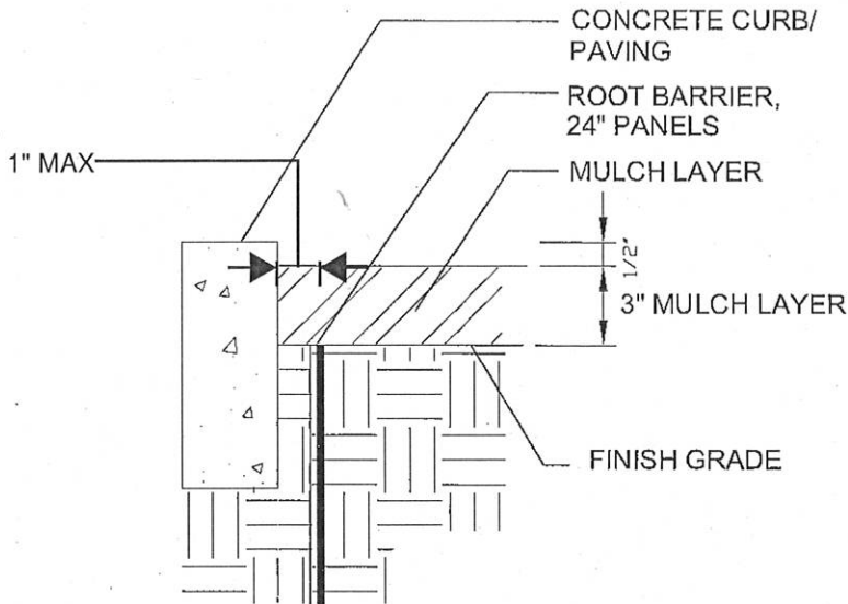
LINEAR ROOT BARRIER SECTION
